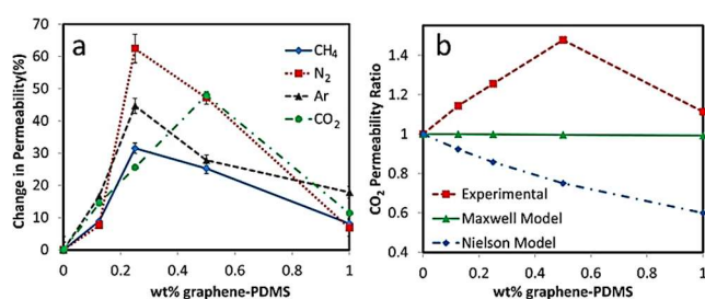
Figure 6. (a) change in permeability for gas species with graphene concentration; (b) experimental data, Maxwell model & Nielson model for CO 2 permeation (0.25 wt.% nanocomposite) [88]. Reproduced with permission from ACS.
