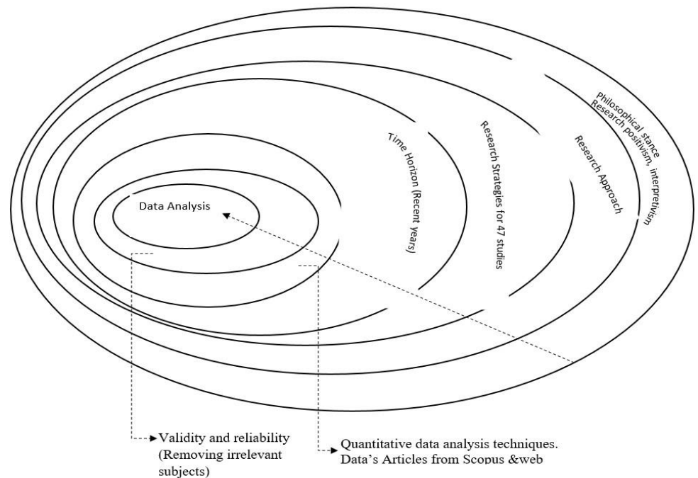
Figure 2. Research onion (Walsham, 2006).
