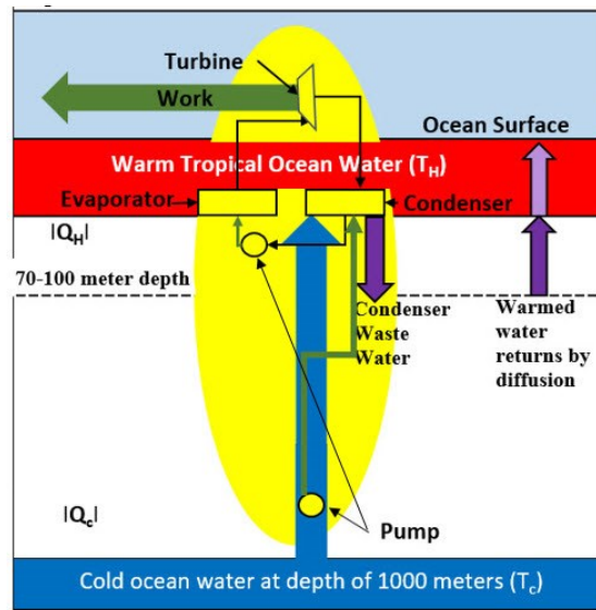
Figure 6. A schematic (not to scale) of conventional OTEC.
