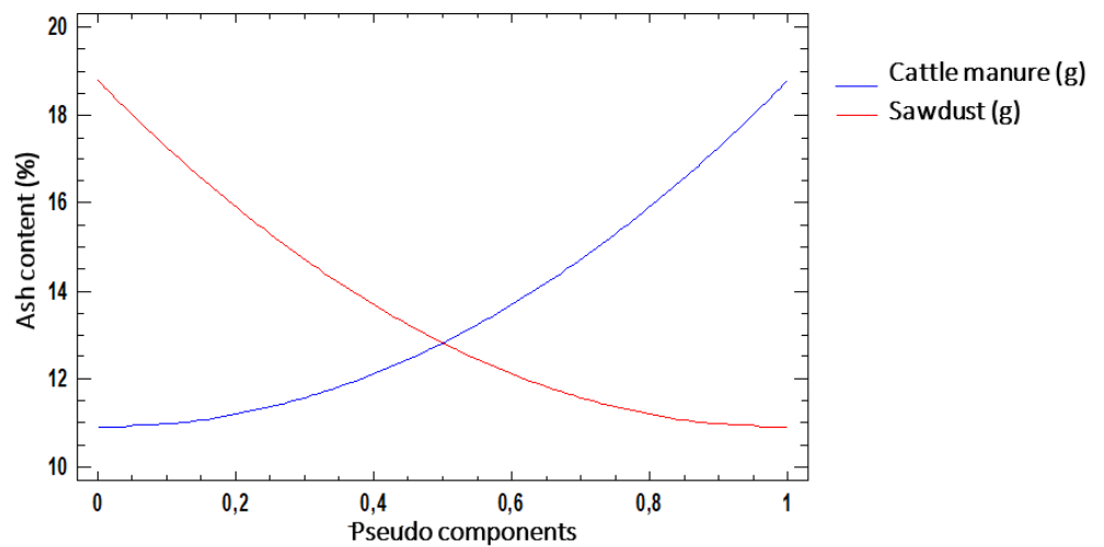
Figure 1. Iso curve response.
