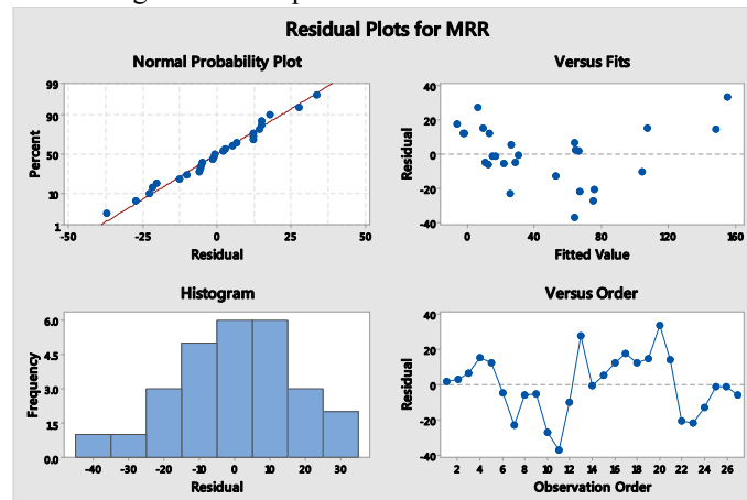
Figure 2; Residual plot for Material removal rate (MRR).
