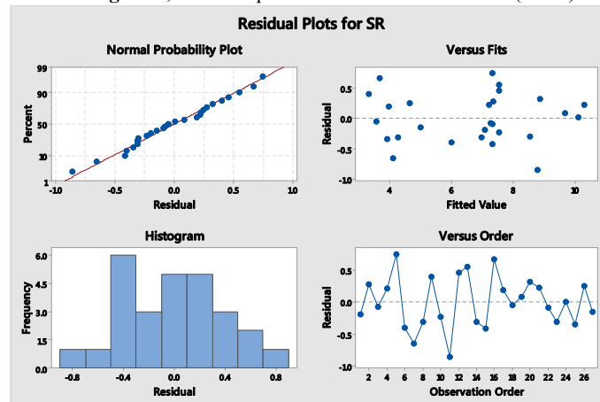
Figure 3; Residual plot for Surface roughness (SR).
