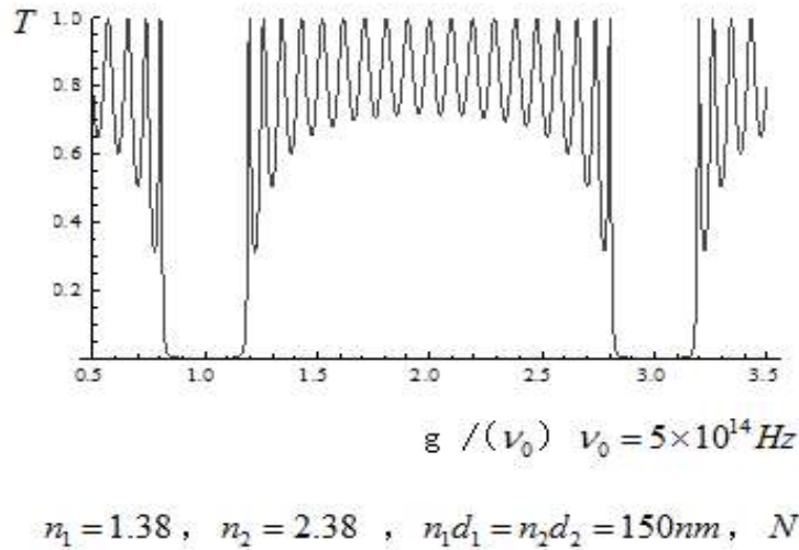
Figure 6. Dimensional photon crystal transmittance
