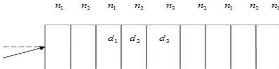
Figure 7. One - Dimensional Photonic Crystals
