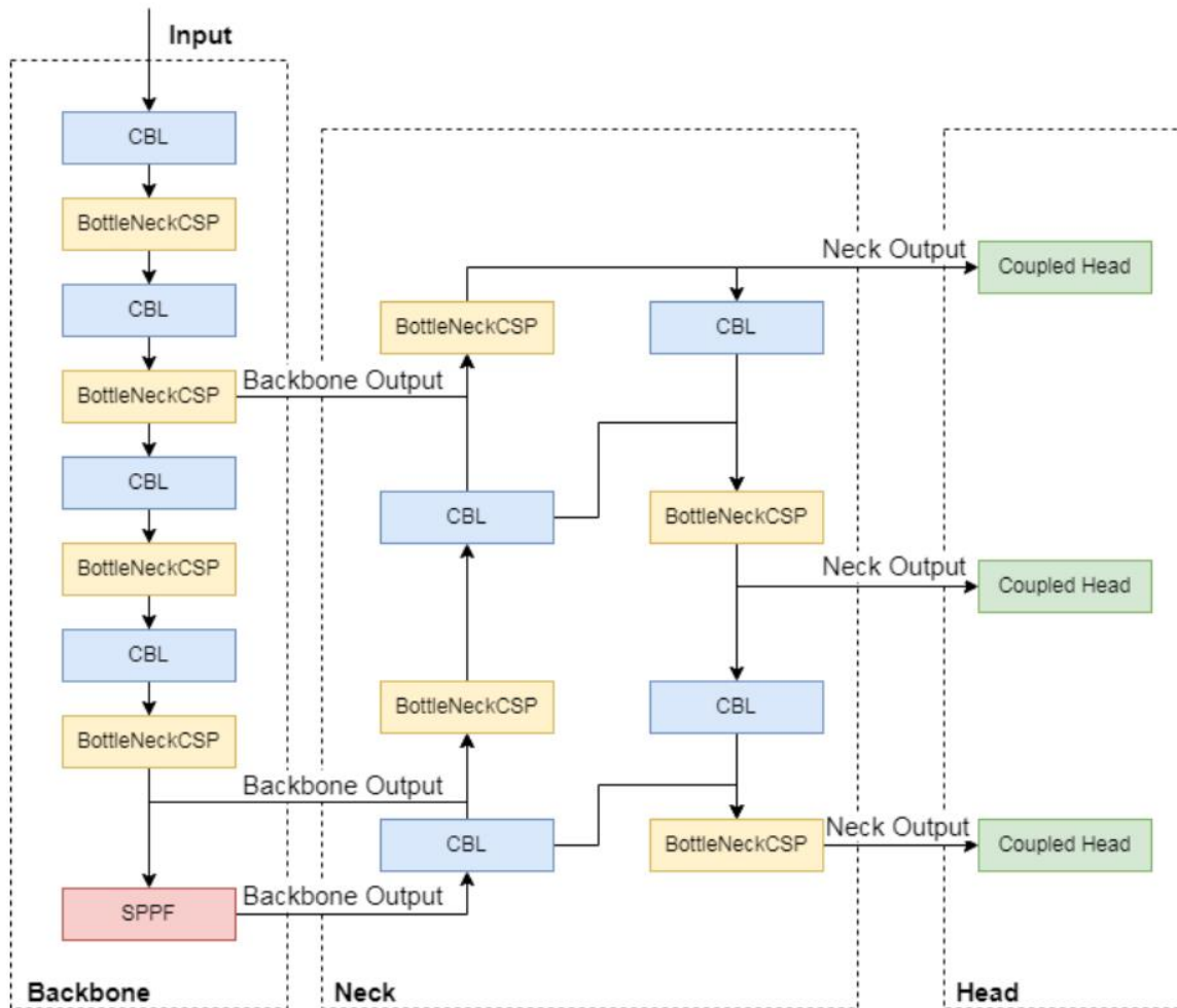
Figure 2. The structure of YOLOv5 [27] .
