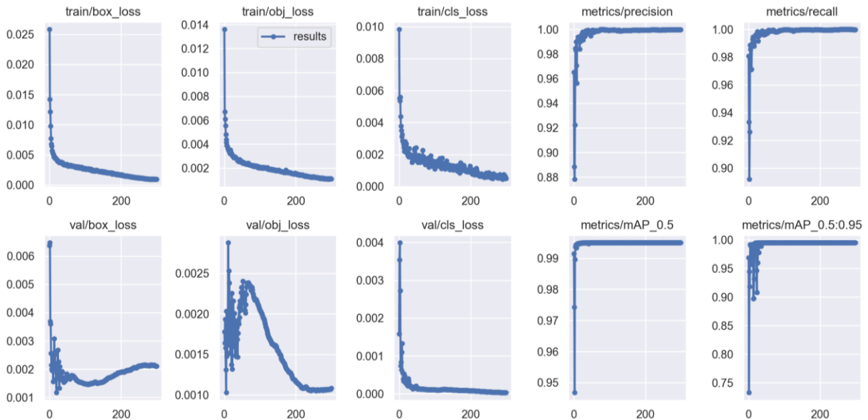
Figure 7. YOLOv5 performance results.
