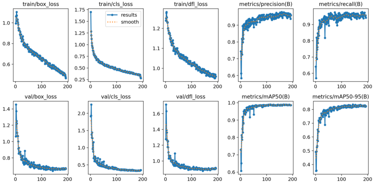
Figure 8. YOLOv8 performance results.
