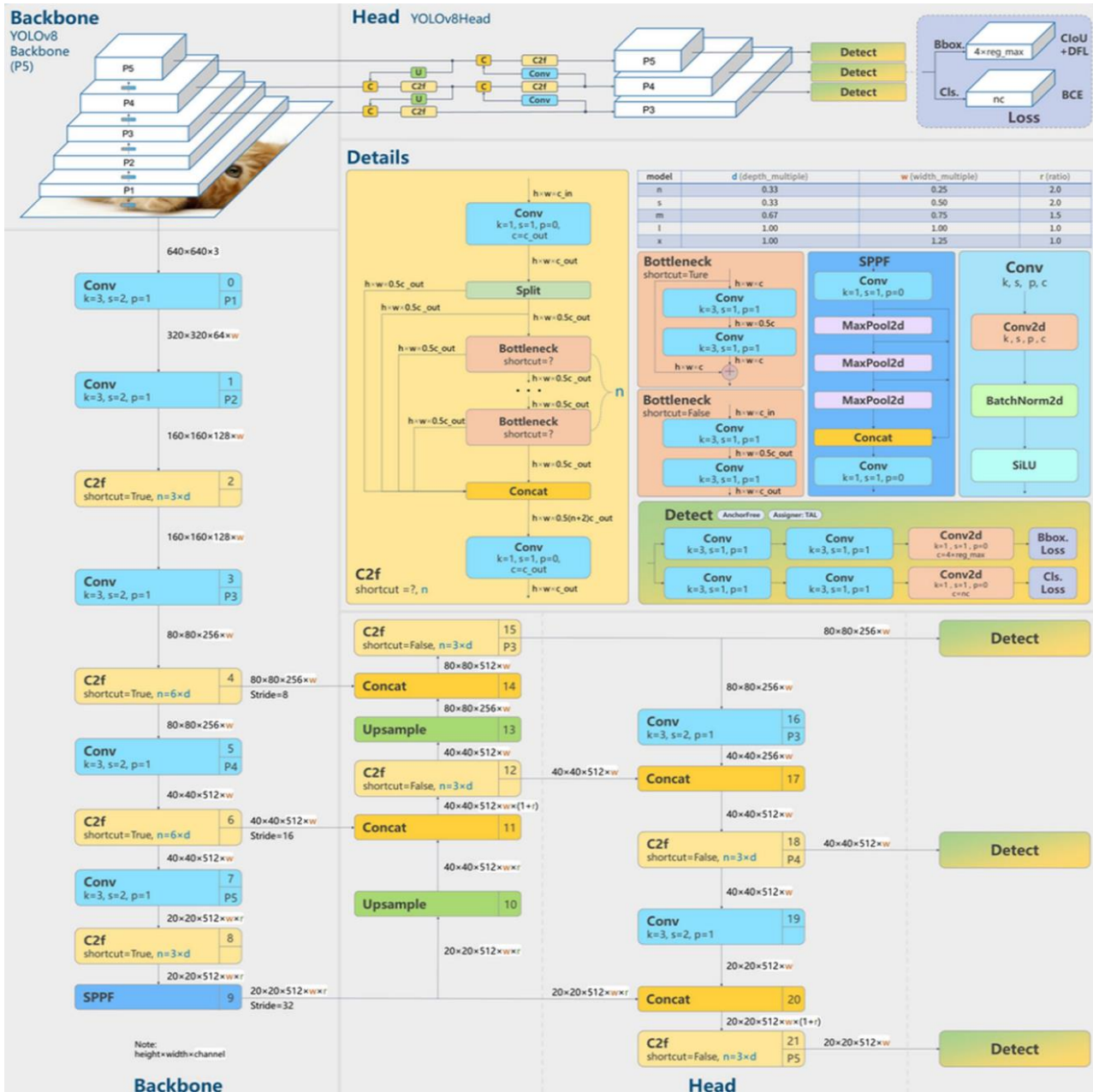
Figure 3. The structure of YOLOv8 [29] .
