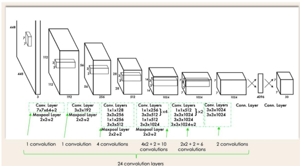
Figure 1. The structure of YOLO [24] .
