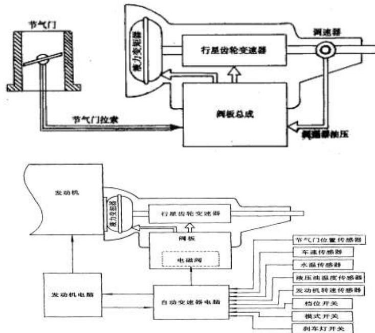
Figure 2. Schematic diagram of the control process of the electronic control automatic transmission
