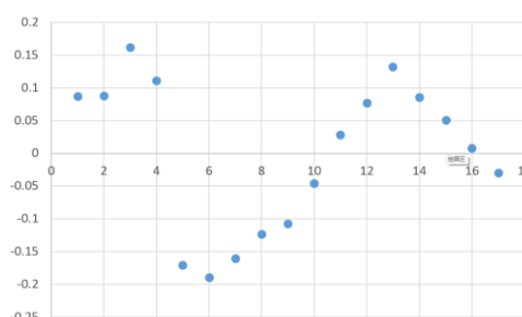
Figure 4. The distribution of residuals for linearized Equation (3).
