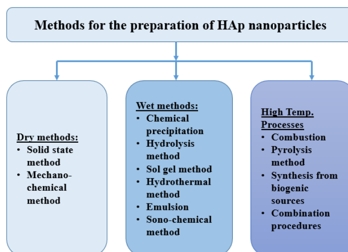
Figure 7. Methods for the preparation of HAp nanoparticles.
